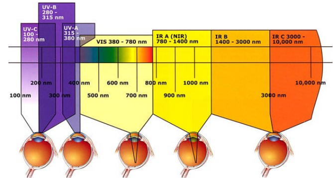
Figure 9. The above table shows the depth of penetration of electromagnetic radiation in the human eye.
