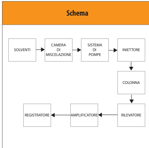
12.13 - Schema HPLC
