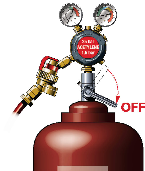
Figure 5 Cylinder head
